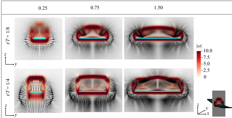
Figure 4. Velocity vectors coloured by the vorticity magnitude at t/T = 1/8 , and t/T = 1/4 for AR = 0.25 , AR = 0.75 and AR = 1.50 at the initial upswEEP cycle and at position x = L/2 .
