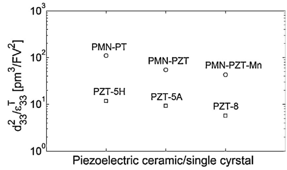
Fig. 2. Comparison of the FOM in low-frequency off-resonant power generation from piezoelectric ceramics (PZT-5A, PZT-5H, PZT-8) and single-crystals (PMN-PT, PMN-PZT).
