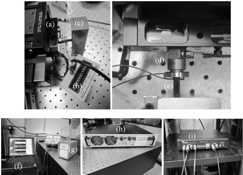
Fig. 3. Experimental setup: (a) electromagnetic shaker; (b) resistor box; (c) stiff fixture; (d) force transducer; (e) piezoelectric stack; (f) computer with data acquisition software; (g) signal conditioner; (h) amplifier; and (i) data acquisition hardware.
