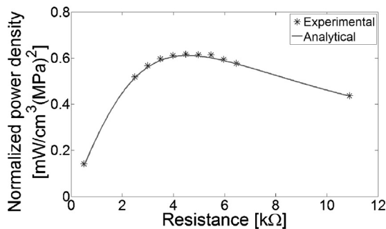
Fig. 7. Power output (normalized with respect to the stack volume and pressure input) versus electrical load resistance under harmonic excitation at 20 Hz.
