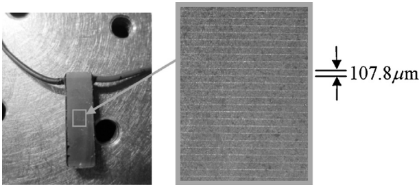
Fig. 4. Close-up picture of the piezoelectric stack and micro-scale picture detail of the layers after the external coat is removed.
