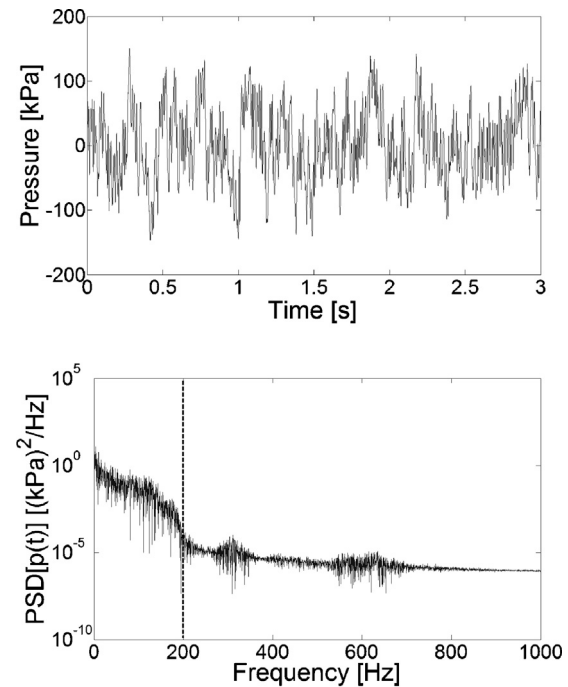
Fig. 9. An experimental time history example for band-limited stochastic pressure excitation applied to the stack (RMS pressure: 58 kPa) and its PSD.
